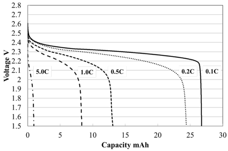
— Discharging (current dependency 25°C) —
