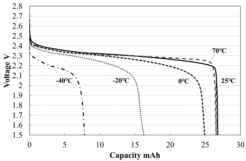
— Discharging (temperature characteristics) —
